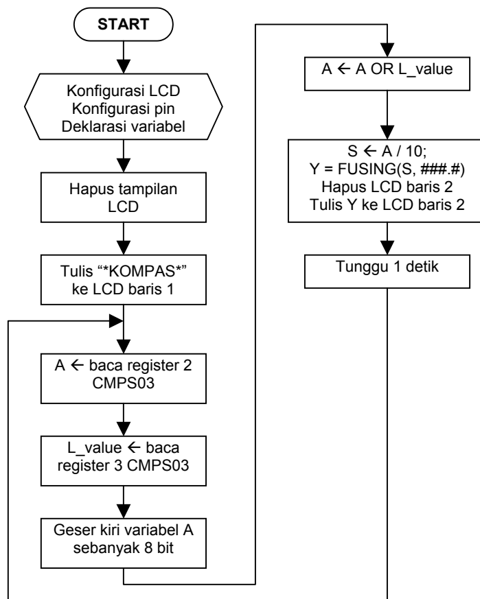
Gambar 6 Flowchart Program i2c_final.bas
