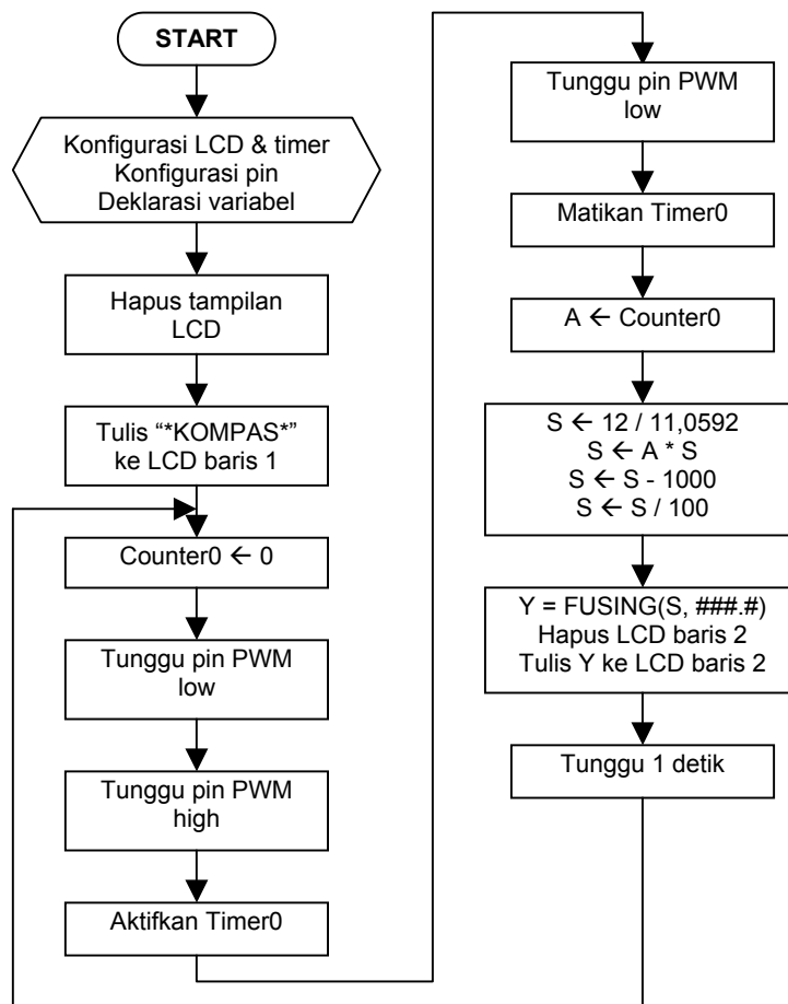
Gambar 7 Flowchart Program pwm_final.bas
